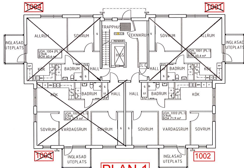
PLAN 1
